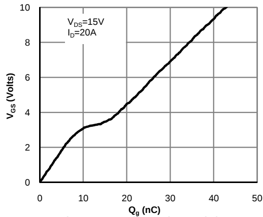
Figure 7: Gate-Charge Characteristics
