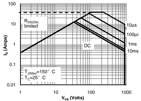
Figure 10: Maximum Forward Biased Safe Operating Area for AOK10N90 (Note F)
