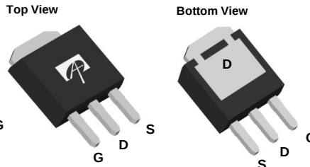
TO-251B IPAK: AOI516/AOY516
