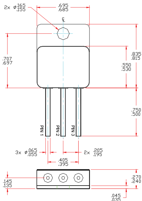
Case Outline: TO-258
