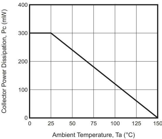
Fig.8 - P_C — T_a
