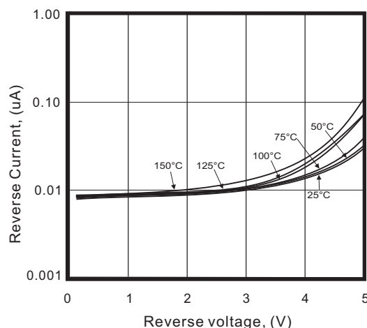
Fig.4 - Reverse characteristics
