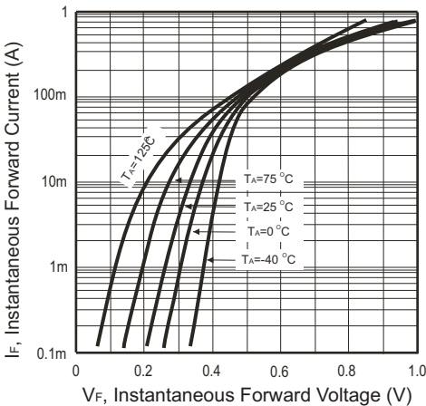
Fig.1 Forward Characteristics
