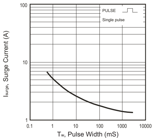
Fig.5 - Surge Current Characteristics
