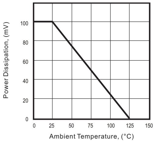
Fig.3 - Derating Curve
