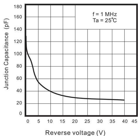
Fig.3 Junction Capacitance
