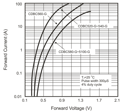
Fig.2 Forward Characteristics
