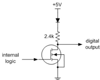
Digital Output Port Circuit:
