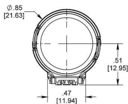
S4 Single-Ended Miniature Optical Shaft Encoder
