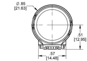
S4 Differential Miniature Optical Shaft Encoder
