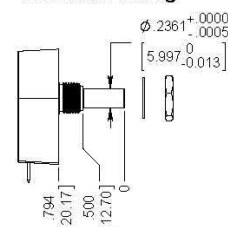
6mm Ball Bearing
