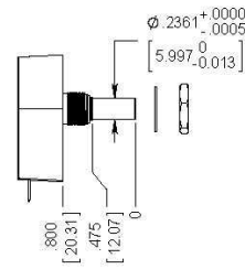
6mm Sleeve Bushing
