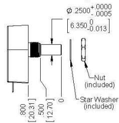
1/4" Sleeve Bushing
