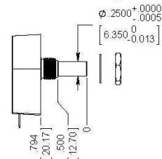
1/4" Ball Bearing
