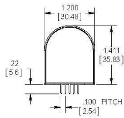
S1 Optical Shaft Encoder Drawing
