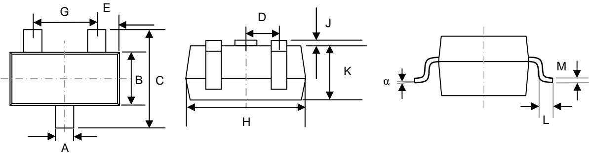
DIMENSIONS (MM)
