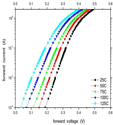
Fig.1 Typical forward I-V
