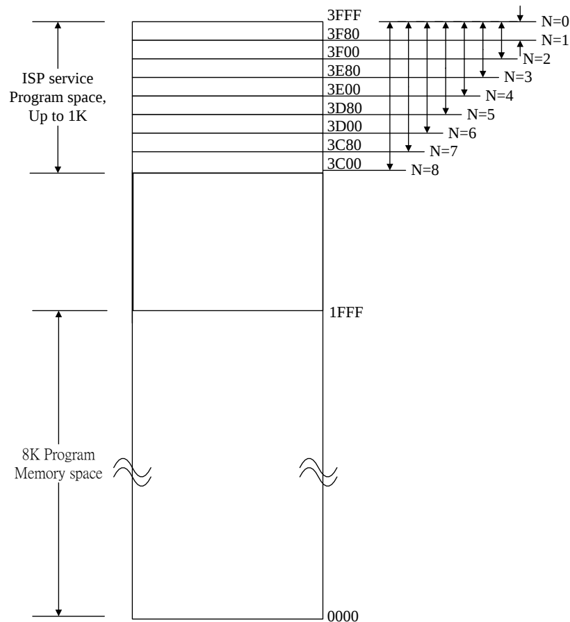
Fig. 3-1: SM39R16A3 programmable Flash
