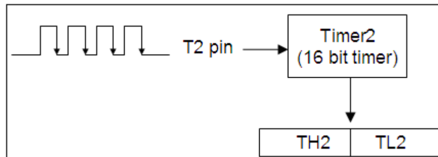
Fig. 7-2: Event counter mode function
