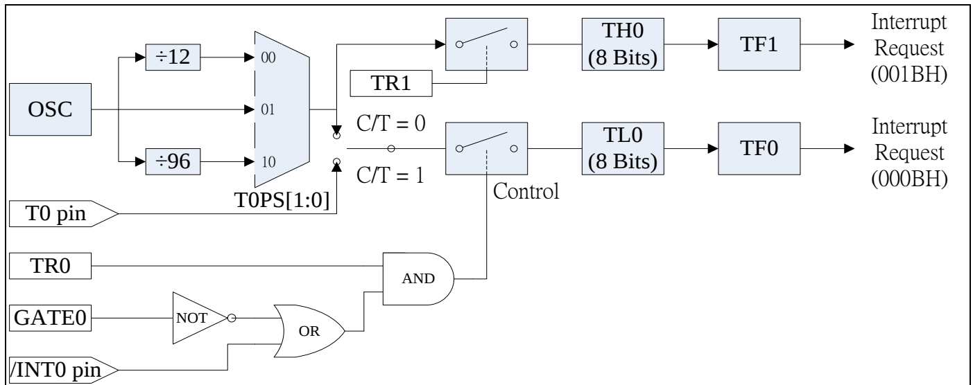
Fig. 6-4: Mode 3 - two independent 8 bit Timers / Counters (Only Timer 0)
