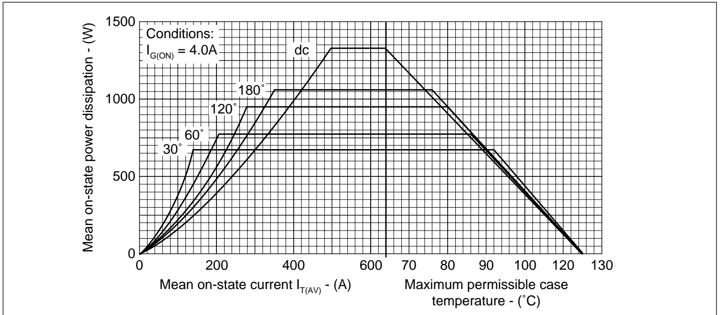
Fig.6 Steady state rectangular wave conduction loss - double side cooled
