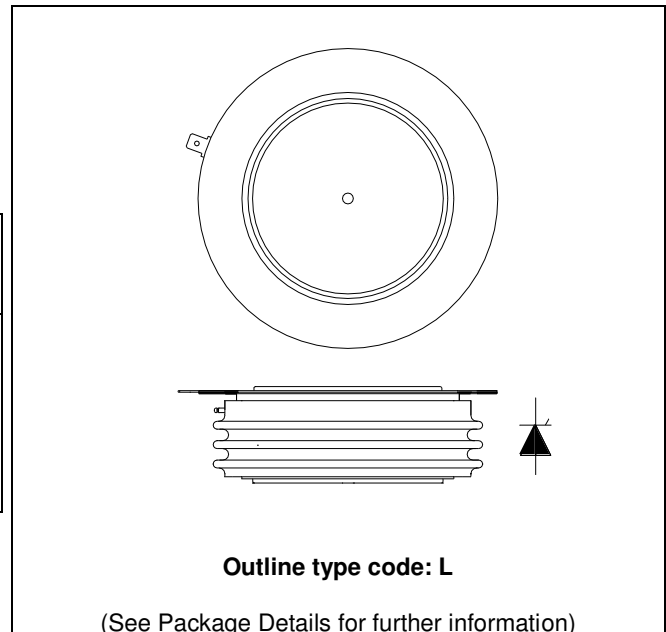
Fig. 1 Package outline
