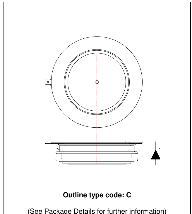
Fig. 1 Package outline
