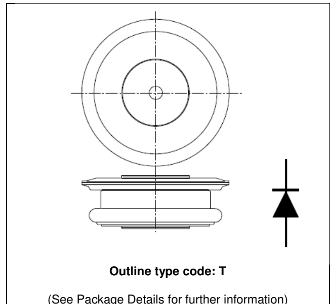
Fig. 1 Package outline
