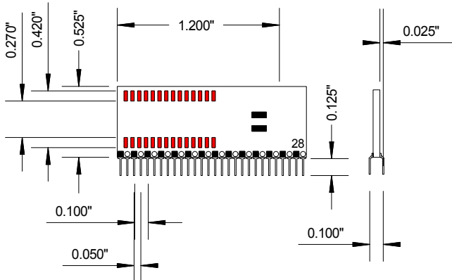
AK28Z-W 28 PIN WIDE SOIC TO ZIP
