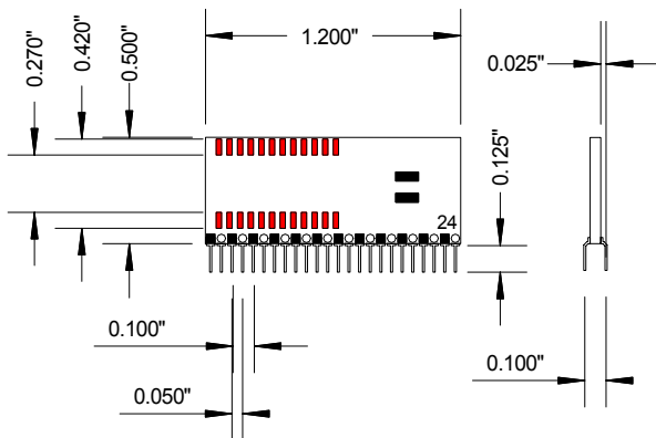
AK24Z-W 24 PIN WIDE SOIC TO ZIP
