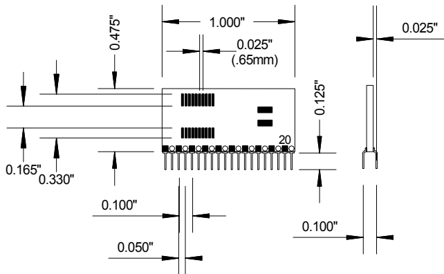
AK20Z-QSOP 20 PIN QSOP OR SSOP TO ZIP
