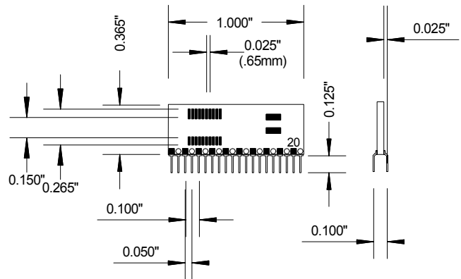
AK20Z-QSOP-LH 20 PIN QSOP OR SSOP TO LOW HEIGHT ZIP
