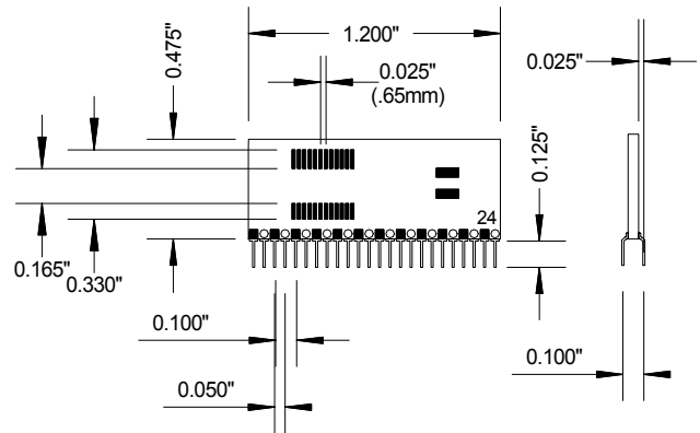
AK24Z-QSOP 24 PIN QSOP OR SSOP TO ZIP
