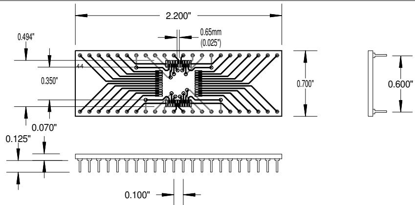
AK44D600-QFP .65mm QFP .65mm PITCH TO 44 PIN DIP
