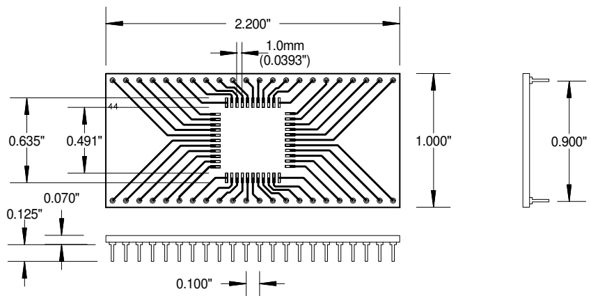
AK44D900-QFP 1.0mm QFP 1.0mm PITCH TO 44 PIN DIP
