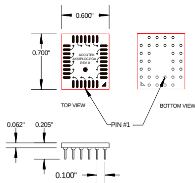
AK32PLCC-PGA 32 PIN PLCC TO PIN GRID ARRAY
