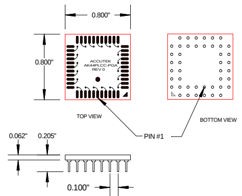
AK44PLCC-PGA 44 PIN PLCC TO PIN GRID ARRAY
