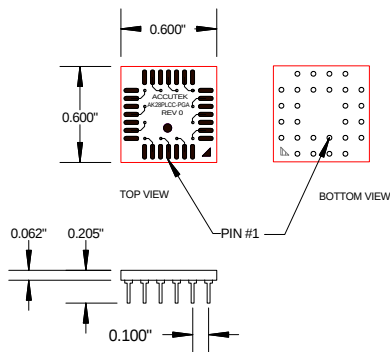
AK28PLCC-PGA 28 PIN PLCC TO PIN GRID ARRAY
