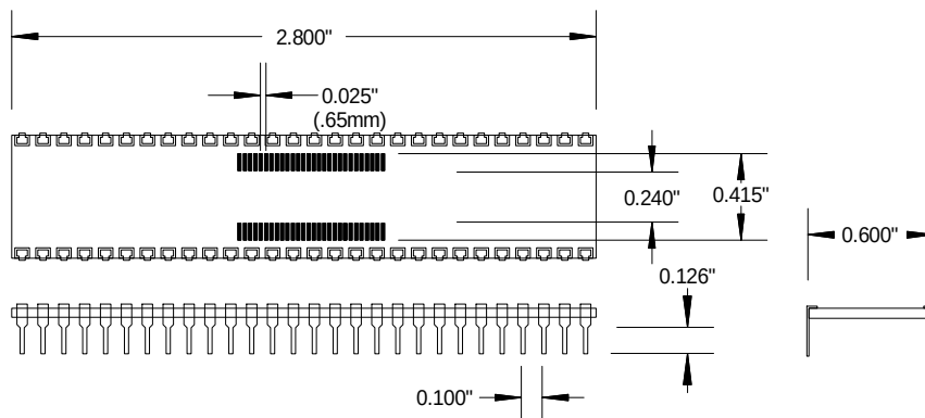
AK56D600-TSSOP.65 .65MM PITCH TSSOP TO 56 PIN DIP
