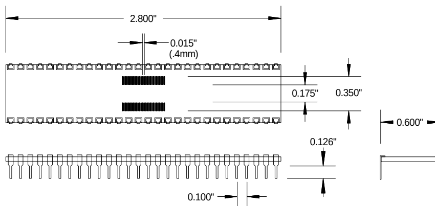
AK56D600-TSSOP.4 .4MM PITCH TSSOP TO 56 PIN DIP
