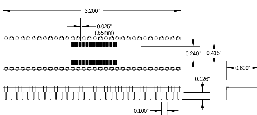
AK64D600-TSSOP.65 .65MM PITCH TSSOP TO 64 PIN DIP
