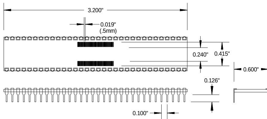
AK64D600-TSSOP.5 .5MM PITCH TSSOP TO 64 PIN DIP
