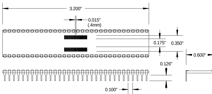
AK64D600-TSSOP.4 .4MM PITCH TSSOP TO 64 PIN DIP
