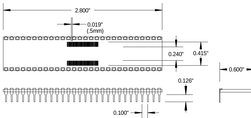
AK56D600-TSSOP.5 .5MM PITCH TSSOP TO 56 PIN DIP
