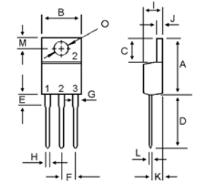
TO-220AB
