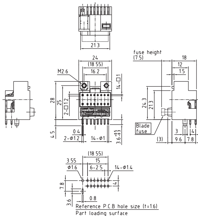
CAM-D50 (Plug)
