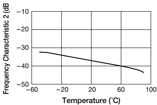
■ Frequency Characteristic 2 vs Temperature (f=27MHz/100kHz)
