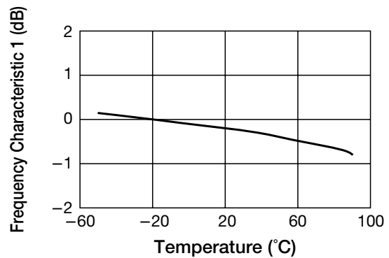
■ Frequency Characteristic 1 vs Temperature (f=6.75MHz/100kHz)
