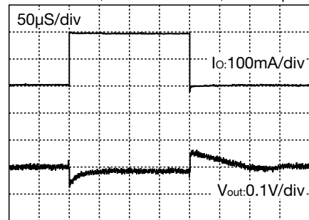
V_{in}=V_{cout}=6.0V, I_o=1mA \leftrightarrow 200mA, C_{out}=2.2\mu F
