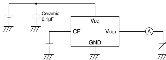
Reverse Current Measuring Circuit
