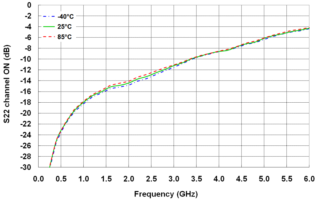
ON state: S22 versus Frequency
