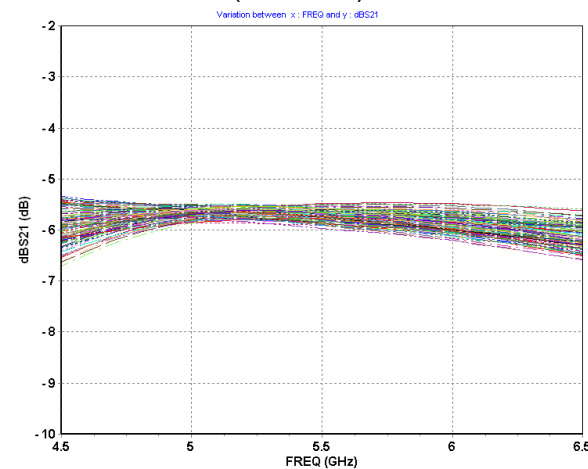
dB(S21) versus frequency (all states)
