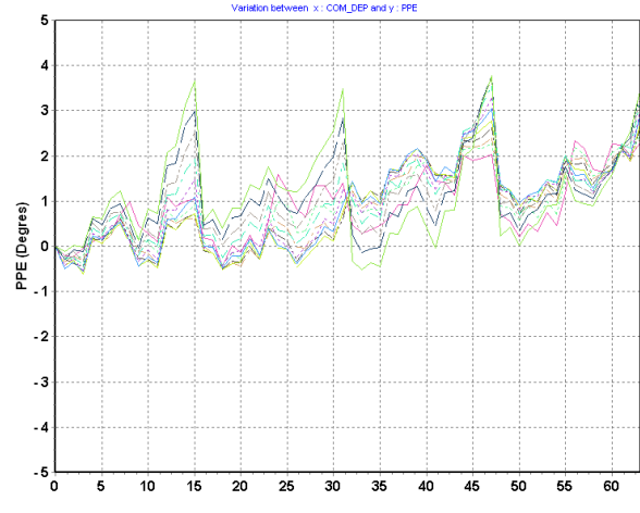
Peak phase error (deg) versus state 5GHz < frequency < 6GHz
