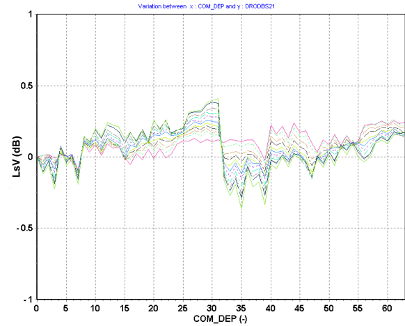
Insertion loss variation (dB) versus state 5GHz < frequency < 6GHz
