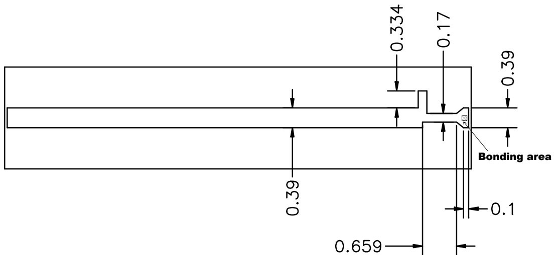
Proposed matching network for a 50Ω transition between OUT2 and a \mu -strip line on DUROID substrate.
