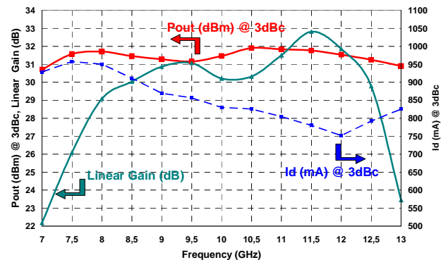
Pout & Id @ 3dB gain compression and Linear Gain (Pulse 25µs 10% Tamb. 20°C)
