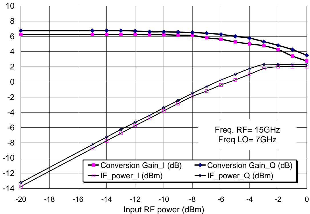
Input RF compression by channel
