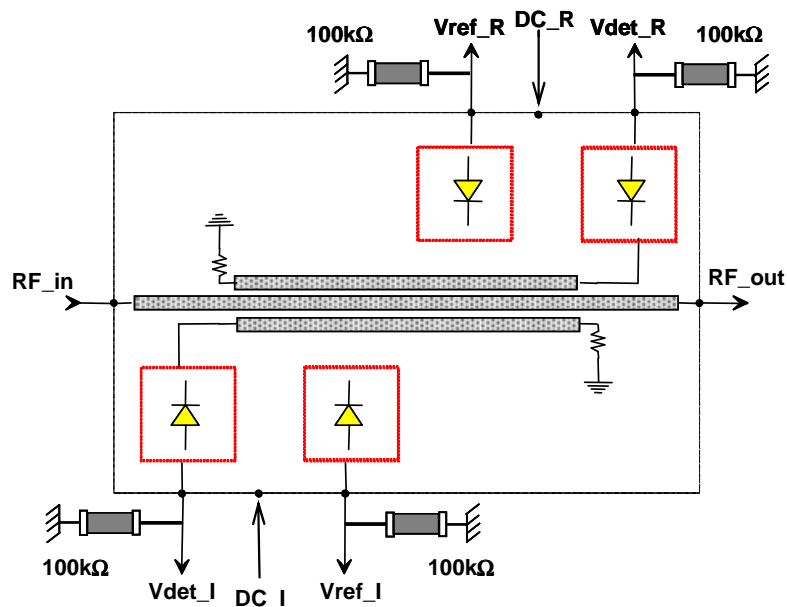
Recommended external resistors assembly
