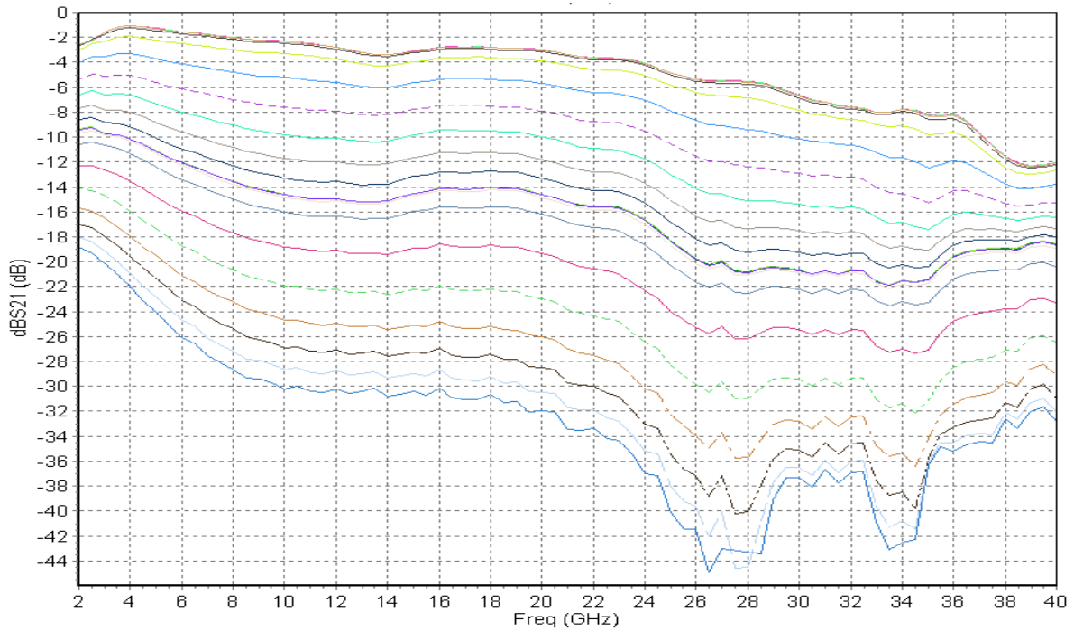
Attenuation versus frequency V1 = -5V to 0V & V2= -5V and after V1= 0V & V2 = -5V to 0V
