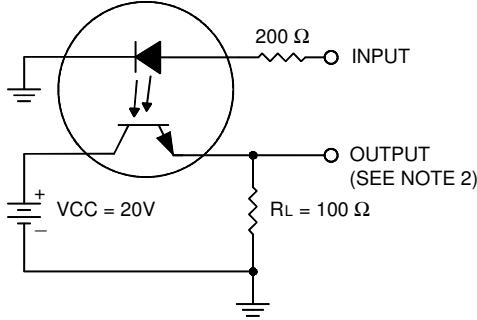
TEST CIRCUIT
