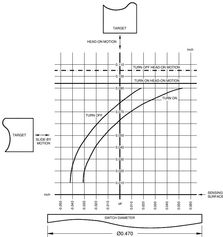
TYPICAL SWITCHING POINT GRAPH
