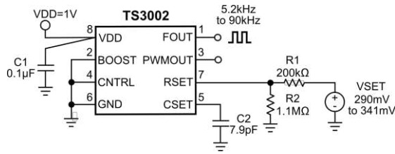
Figure 3: Configuring the TS3002 into a Voltage-Controlled Oscillator.
