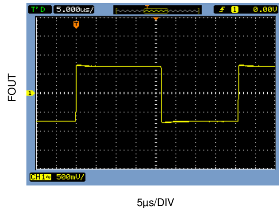
FOUT Transient Response V_{DD} = 1.5V , BOOST = V_{DD} , C_{LOAD} = 47pF
