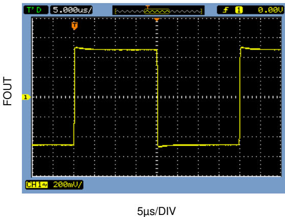
FOUT Transient Response V_{DD} = 1V , BOOST = V_{DD} , C_{LOAD} = 47pF
