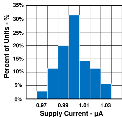
Supply Current Distribution
