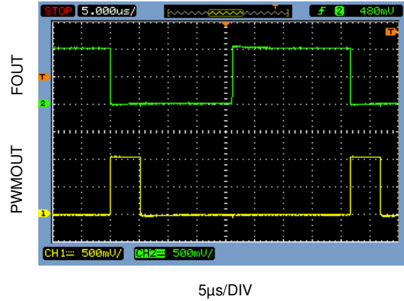
FOUT and PWMOUT Transient Response V_{DD} = 1V , V_{CTRL} = 0.035 \times V_{DD} , BOOST = V_{DD} , C_{LOAD} = 22pF
