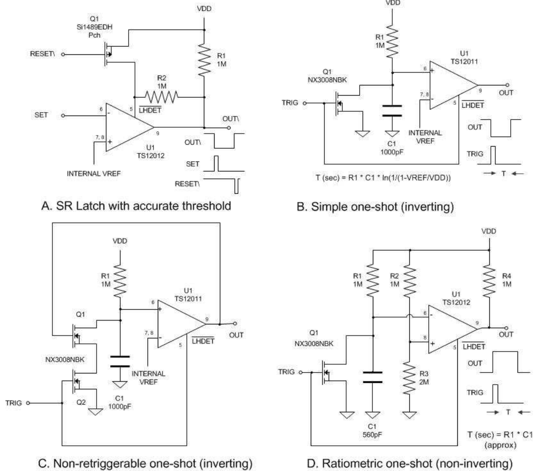
Figure 6. Low-power One-shot and Latch Circuits
