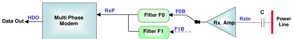
Figure 4.02 – Receive path.
