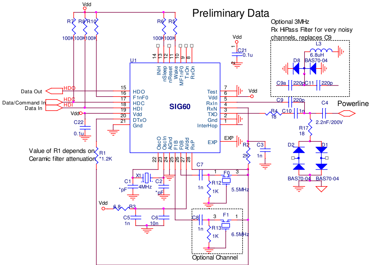
Figure 3.3 – SIG60 schematics example
