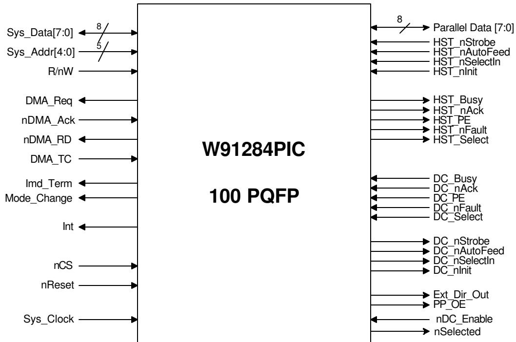
Figure 9 – I/O Signals
