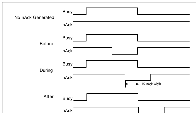
Figure 4 – nAck Position
