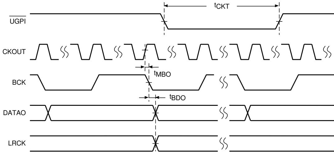
Figure 7.1 AC Characteristics
