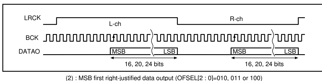
Figure 8.6 Data Output Timing (Normal Mode)
