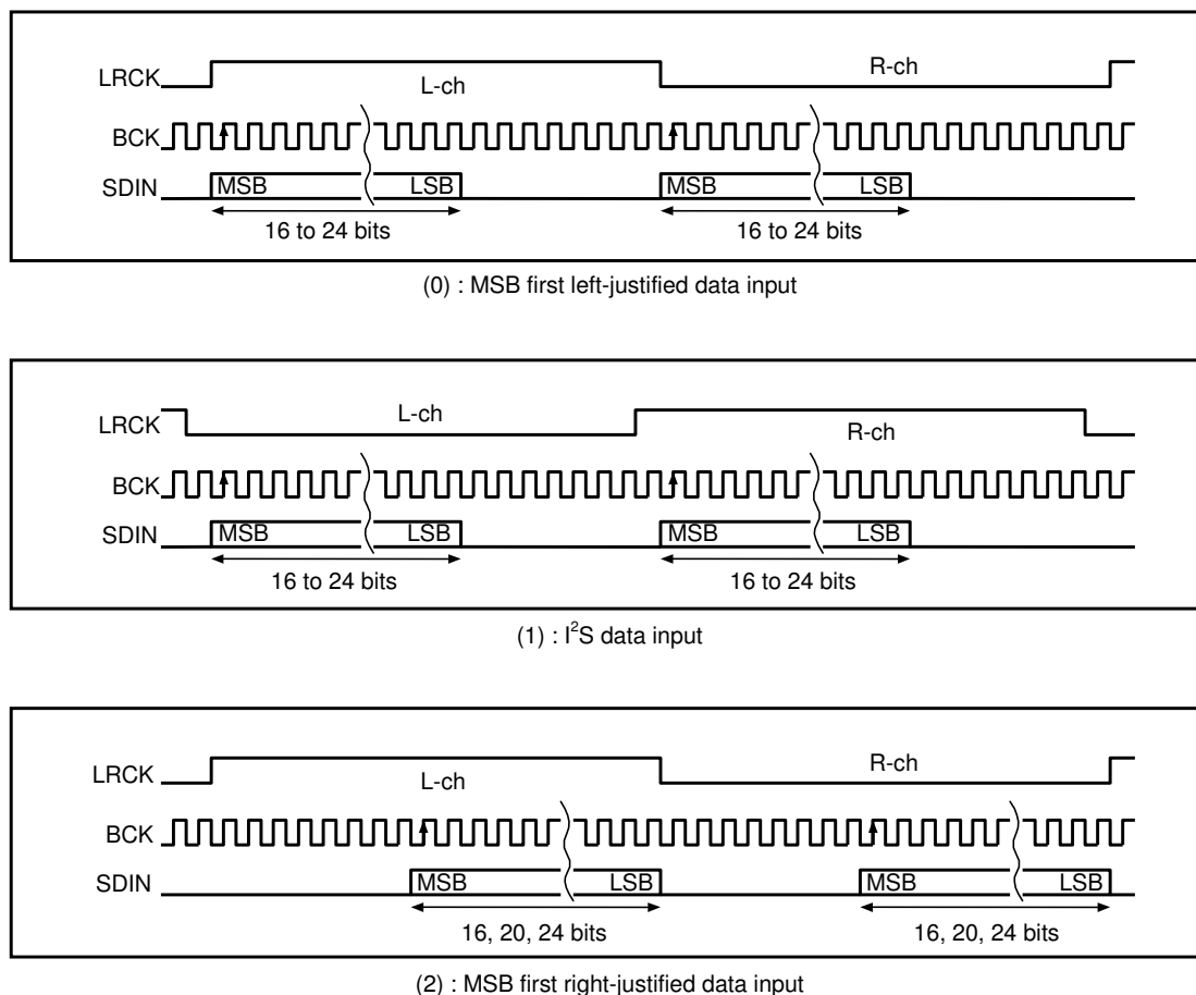
Figure 8.8 Example of Serial Audio Data Input Timing
