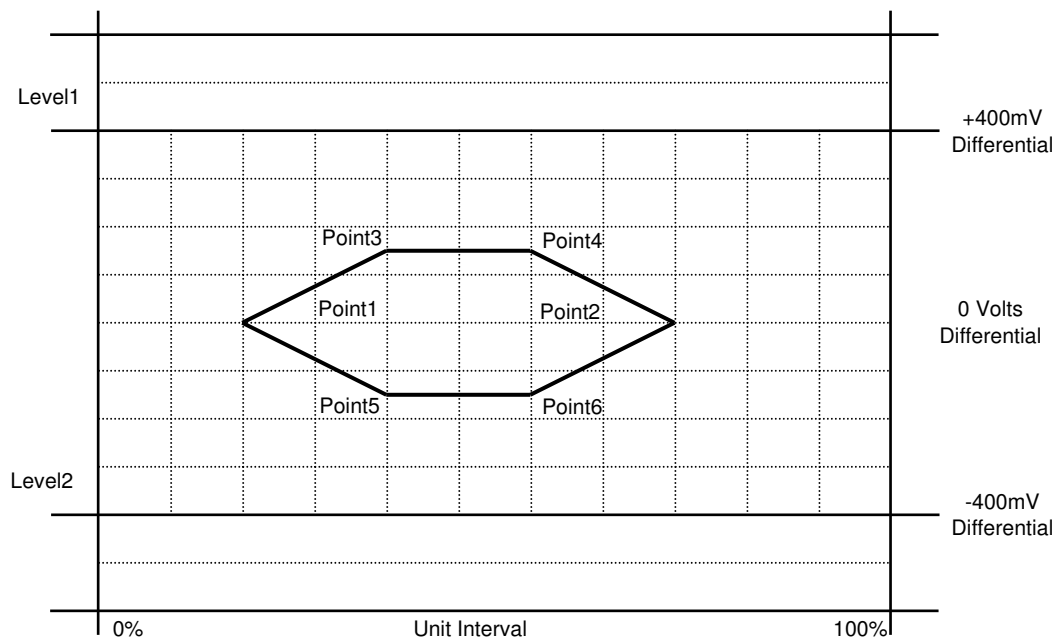
Figure 2.2: Differential Input Sensitivity Range for High-speed
