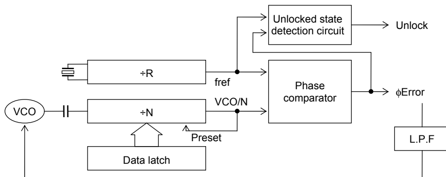
Figure 2 Circuit Structure
