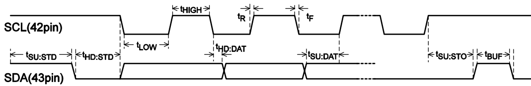
Fig.2 Definition of timing
