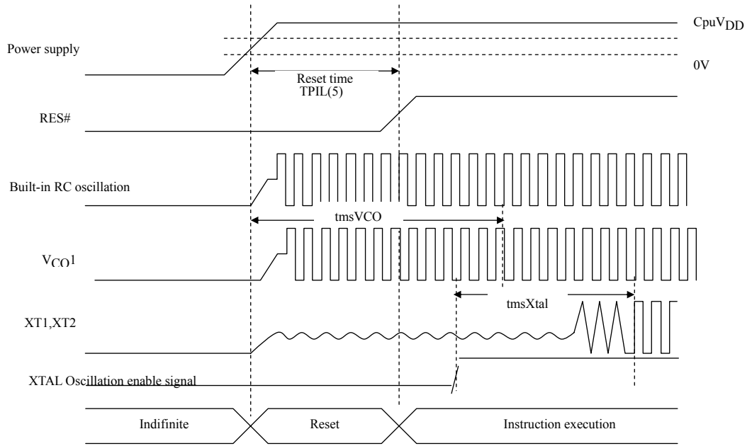
Reset time and oscillation stable time
