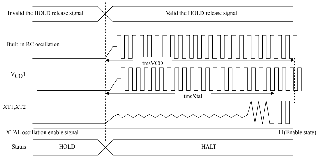
HOLD release signal and oscillation stable time
