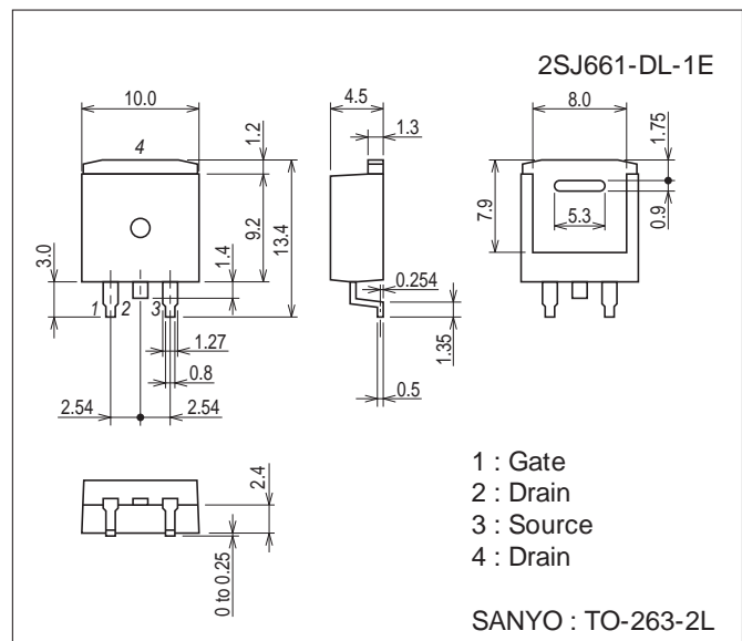
Package Dimensions unit : mm (typ) 7535-001
