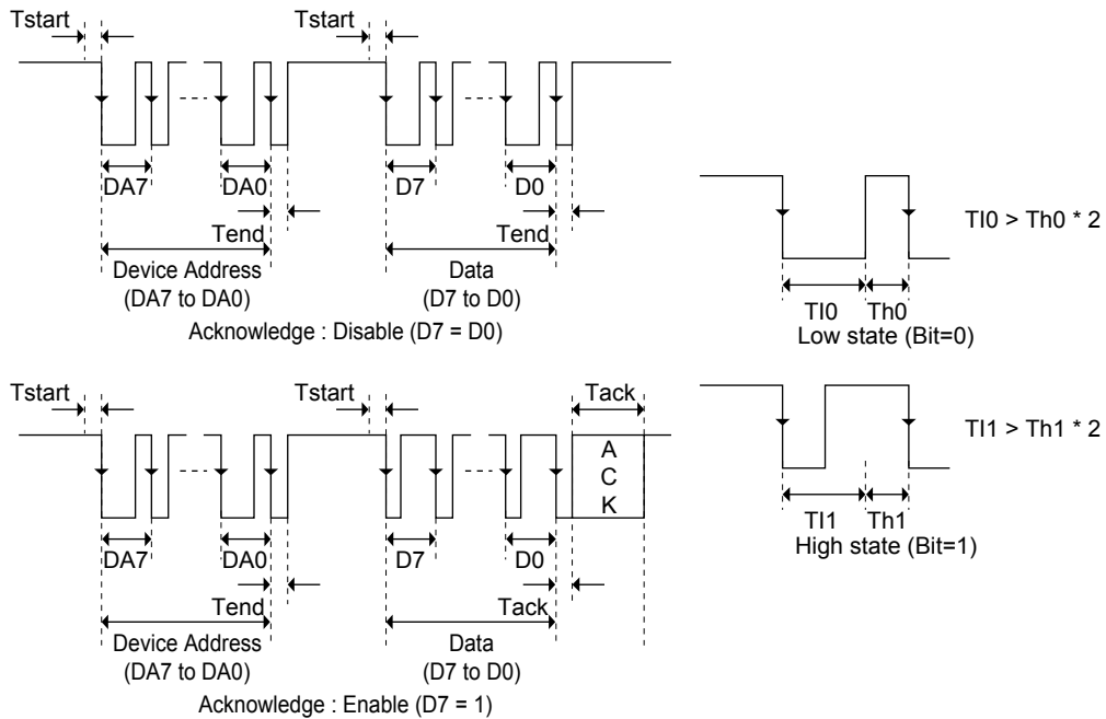
Fig6.Bit detection Diagram
