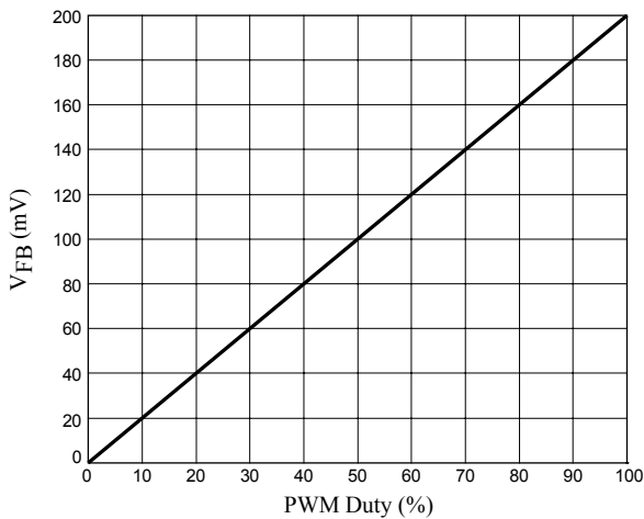
Fig1. V_{FB} vs. PWM Duty (PWM mode)
